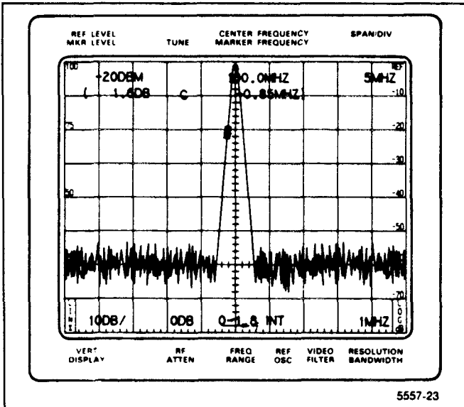
Figure 6-10. Simulated display showing delta marker operation with signal count on a saved display.
