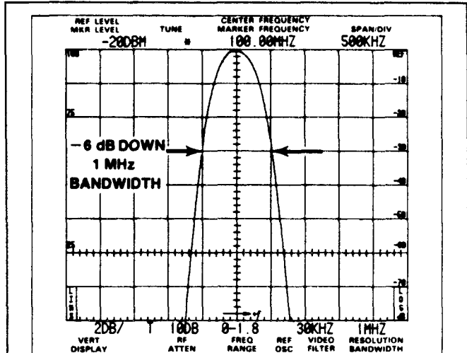
A. Measuring 6dB down bandwidth.
