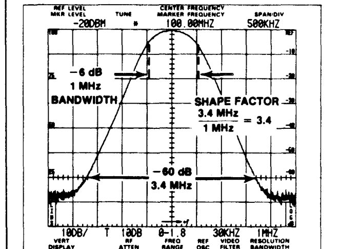
B. Measuring 60dB down bandwidth and computing shape factor.
