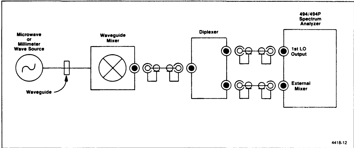
Figure 6-11. Block diagram showing external waveguide mixer installation.
