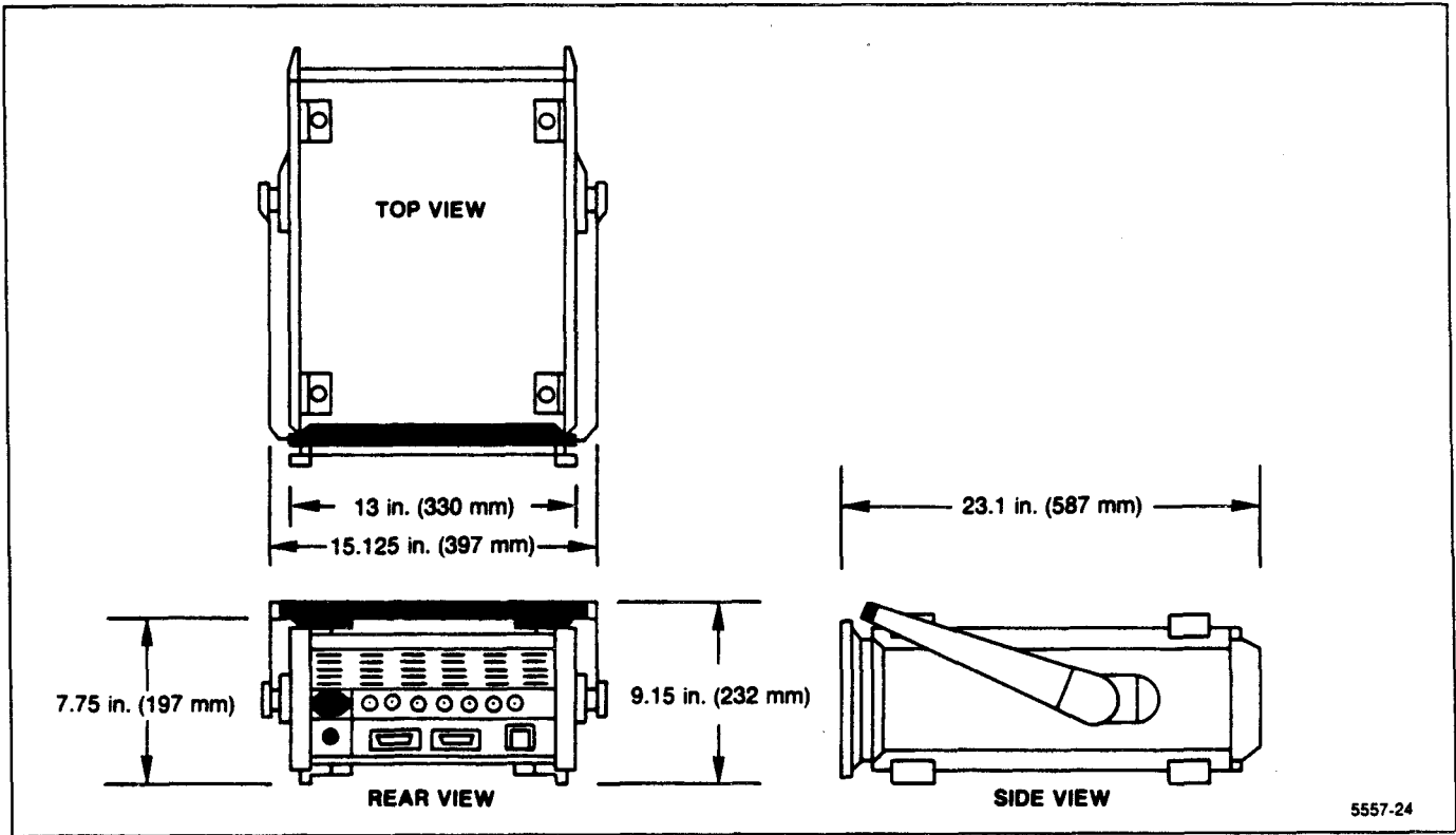
Figure 2-1. Dimensions.
