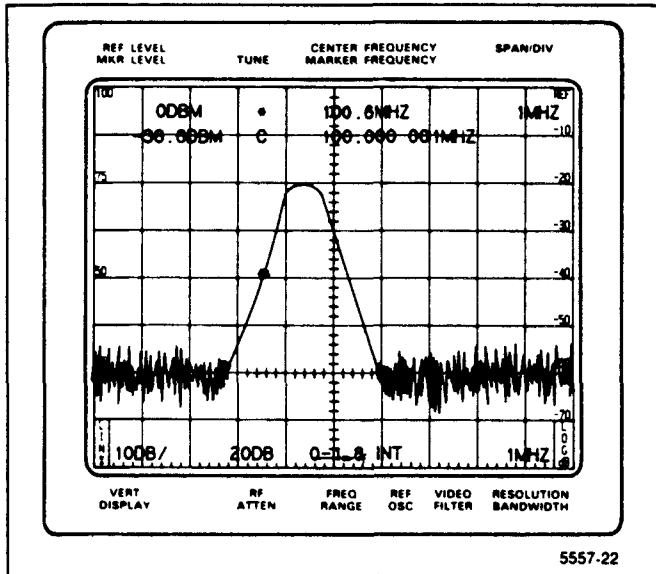
Figure 6-9. Simulated display showing counting being done at the marker while the center frequency is being tuned.
