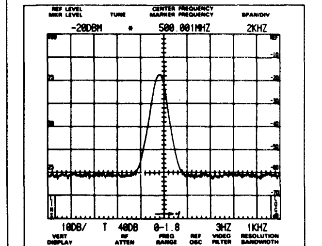
B. Same display with Video Filter activated.
